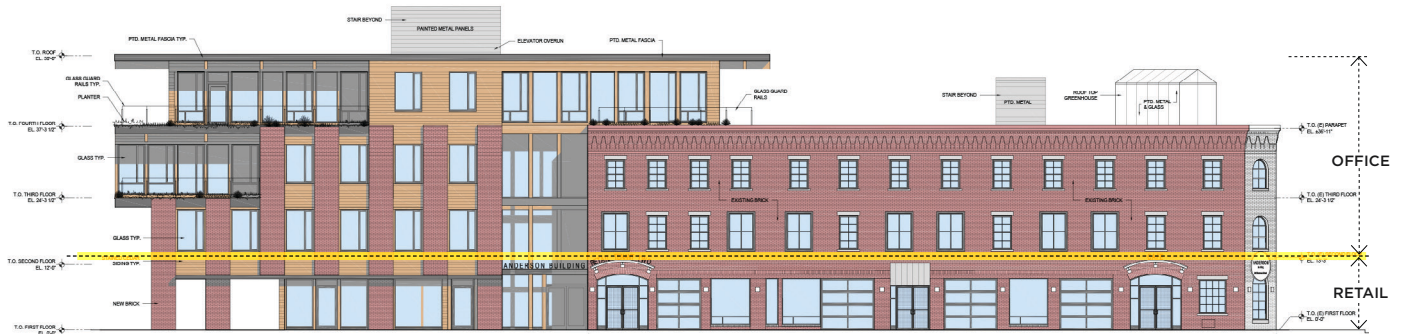
SOUTH ELEVATION (MONMOUTH STREET)
